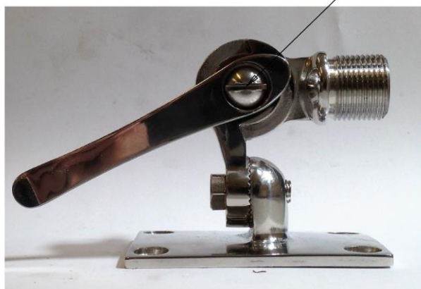
4: Tighten the bolt by 10Nm while keeping the new handle position
