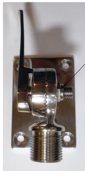
5: Tighten the lock nut by 10Nm while keeping the new handle position
