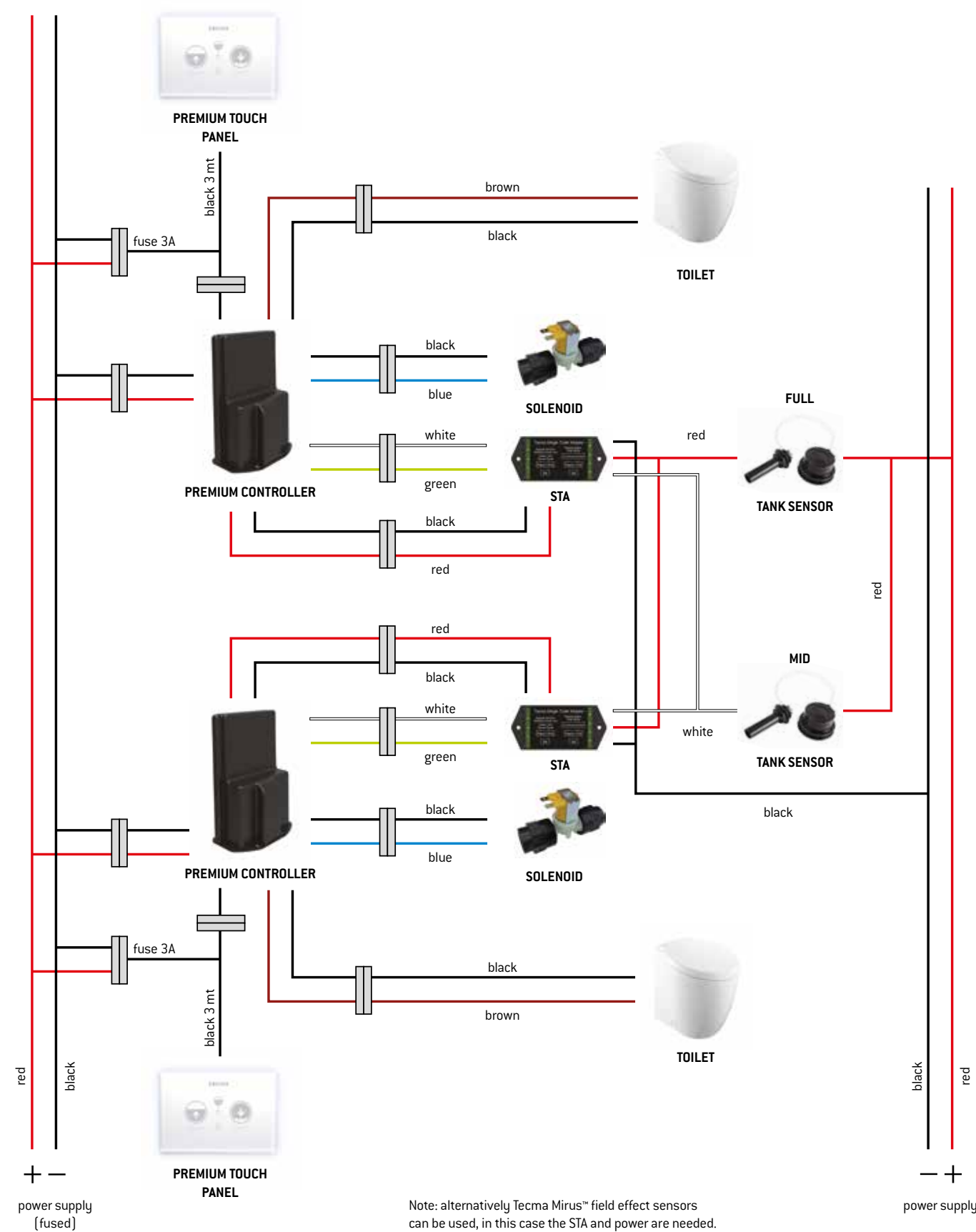
Fresh water wiring - Premium Touch panel
