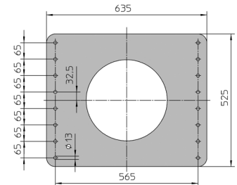
CF-ACV-600-60-7
