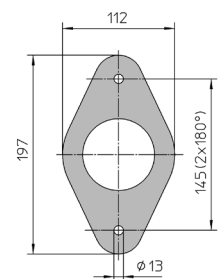
CENTA TB 1
