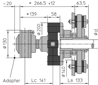
CF-ACV-50-21-3
