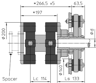
CF-AGM-50-3
